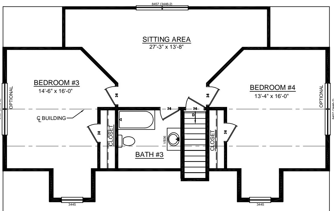
OPTIONAL SECOND FLOOR - SITE BUILT
