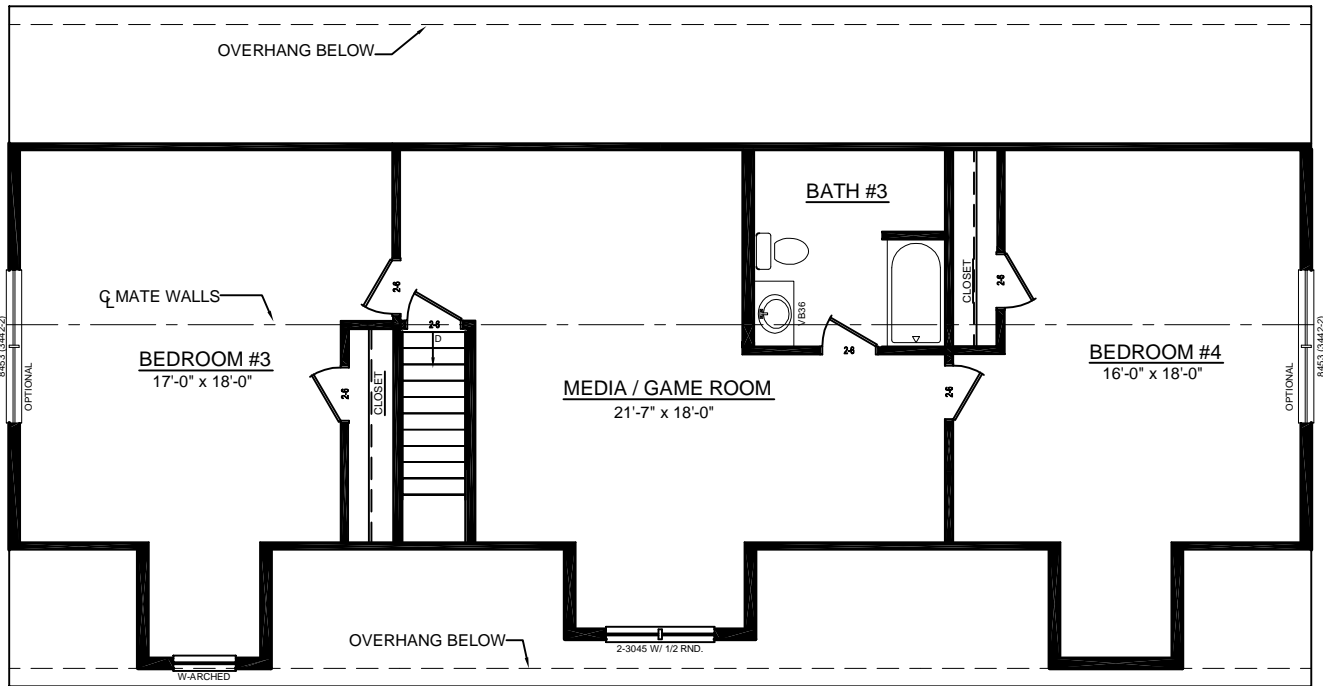
OPTIONAL SECOND FLOOR - SITE BUILT
