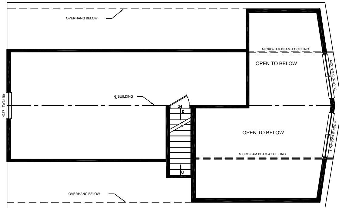
SECOND FLOOR
