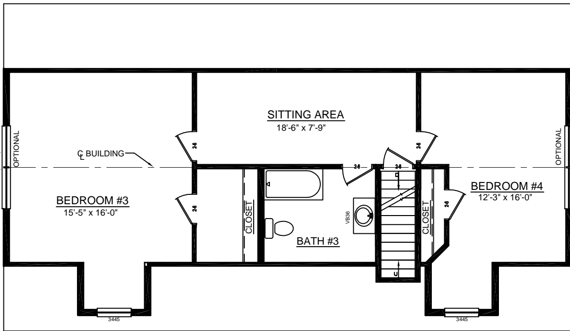
OPTIONAL SECOND FLOOR - SITE BUILT
