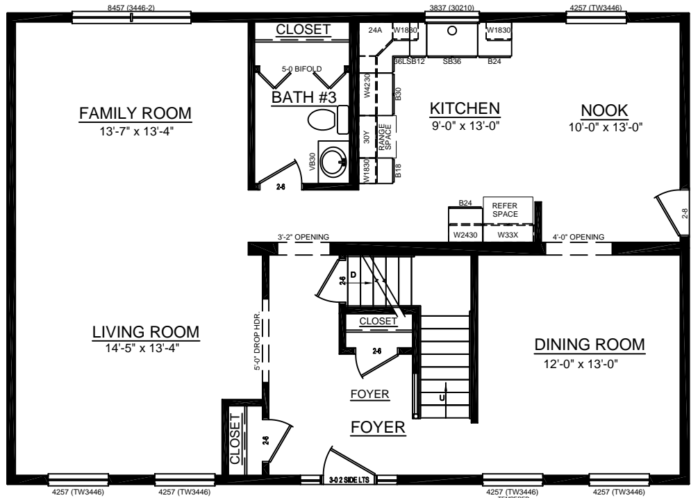
FIRST FLOOR PLAN VIEW
