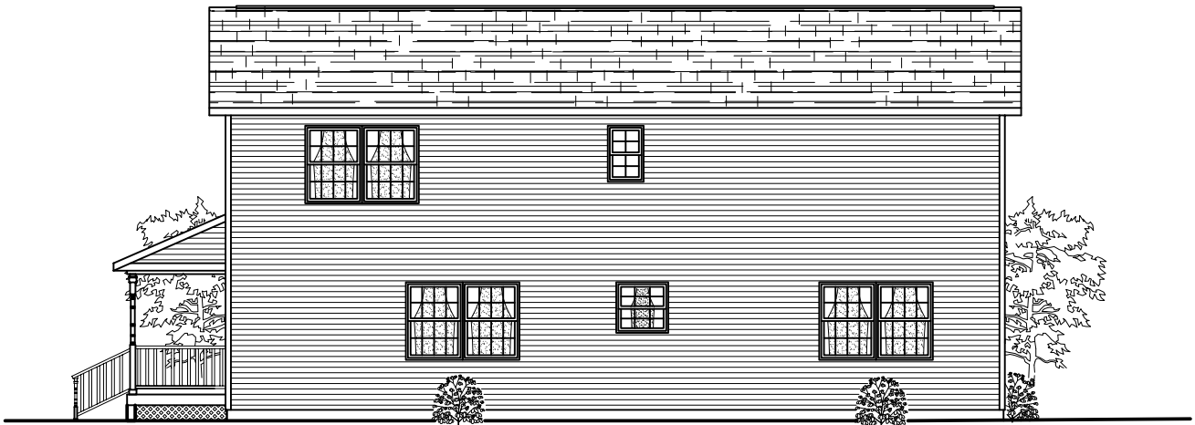
REAR ELEVATION
