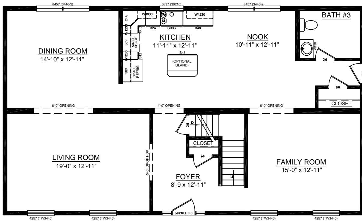
FIRST FLOOR PLAN VIEW
