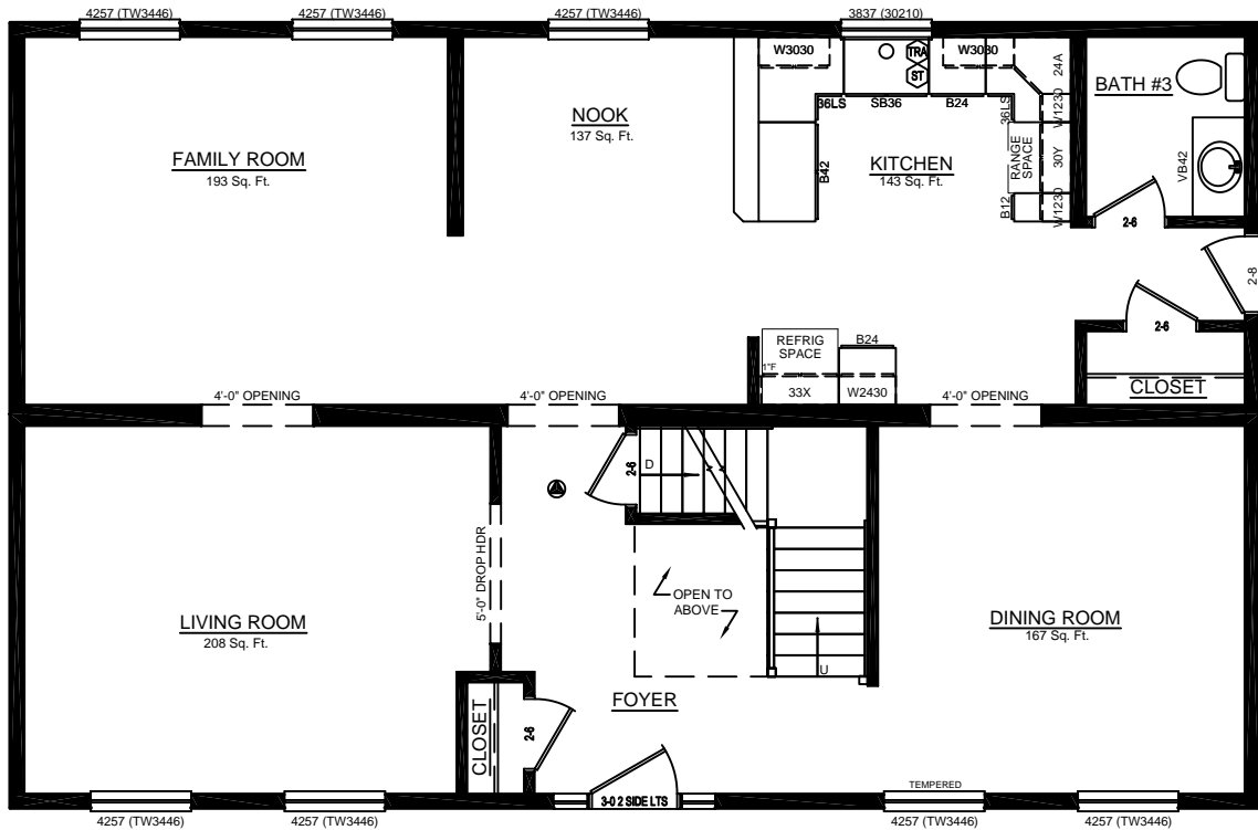
OPTIONAL 1st FI PLAN
