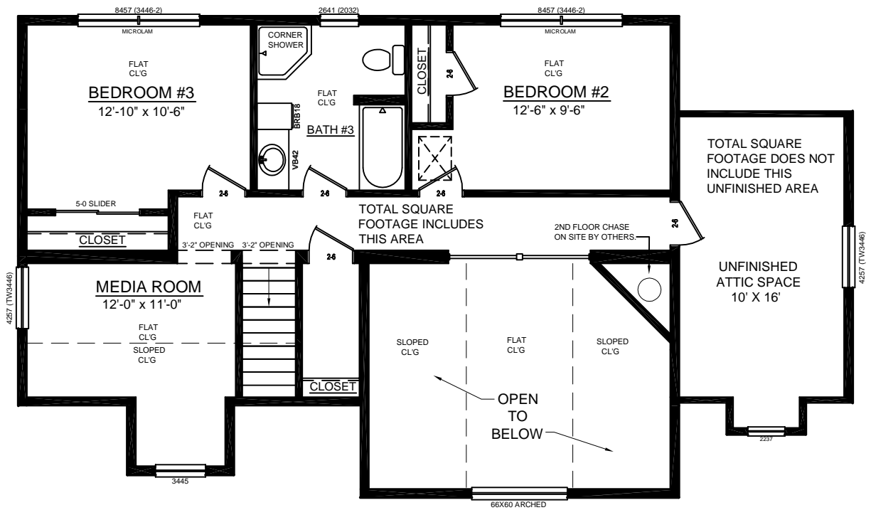
OPTIONAL SECOND FLOOR
