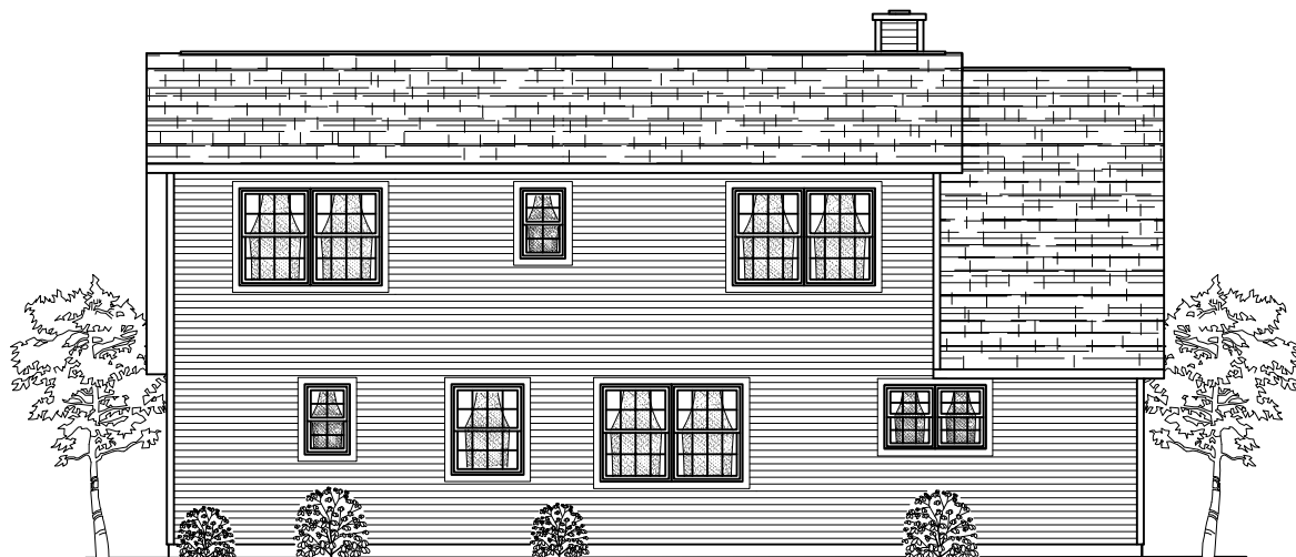
REAR ELEVATION
