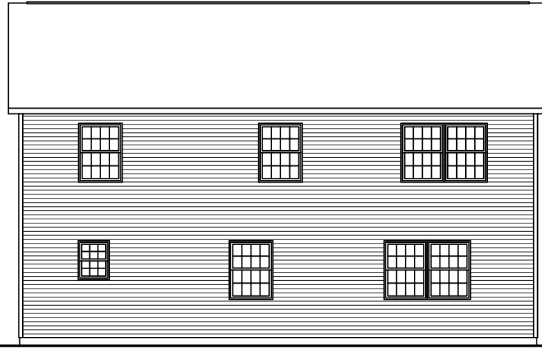
REAR ELEVATION
