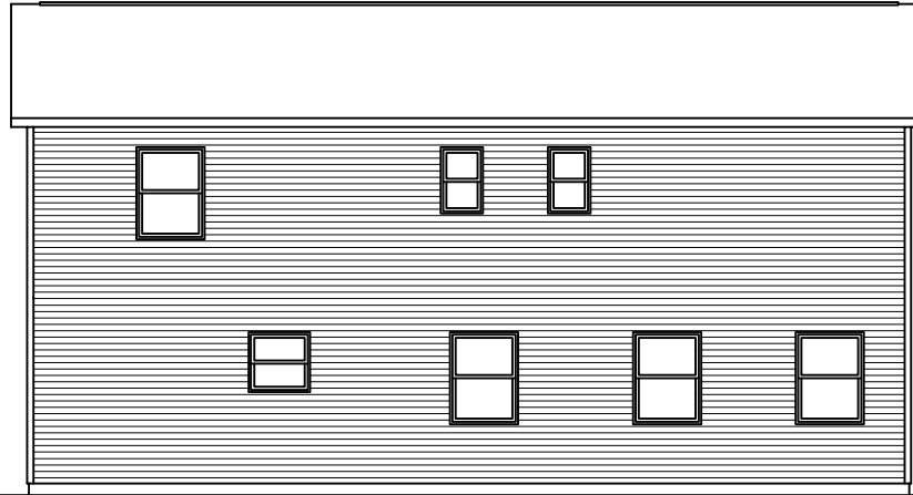
REAR ELEVATION
