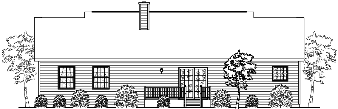
REAR ELEVATION
