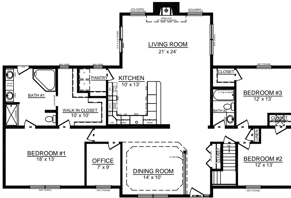
FLOOR PLAN
