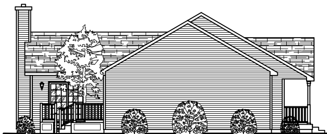
LEFT ELEVATION
