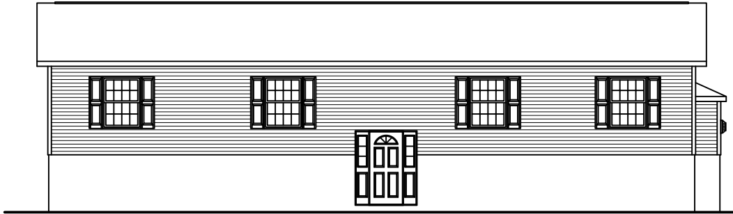
FRONT ELEVATION
