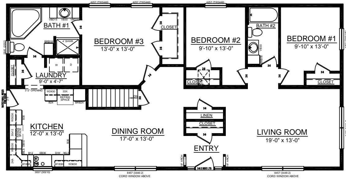
FLOOR PLAN
