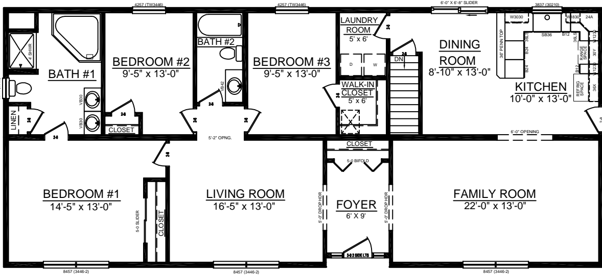
FLOOR PLAN
