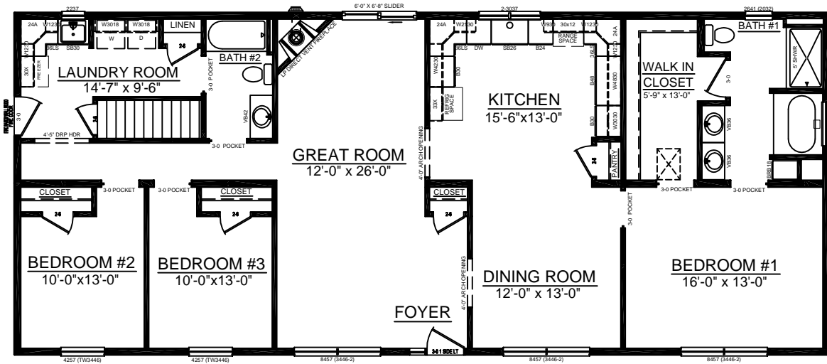
FLOOR PLAN
