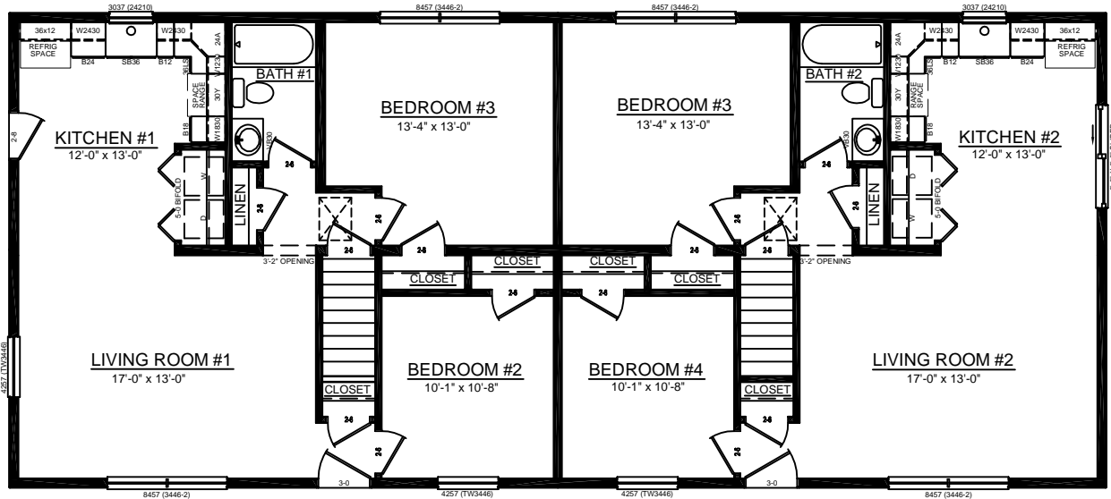
FLOOR PLAN
