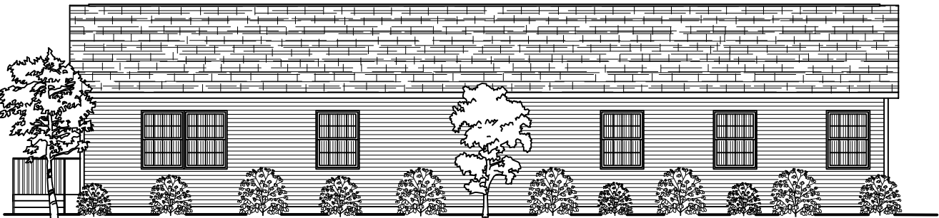
REAR ELEVATION
