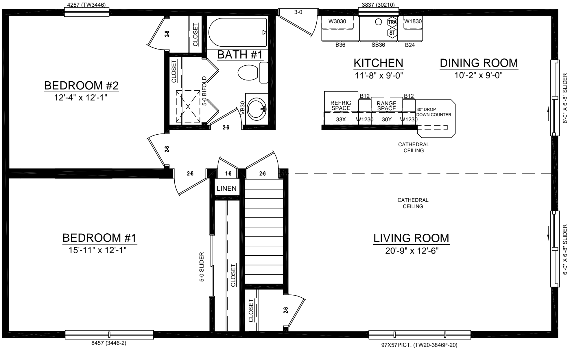
PLAN VIEW
