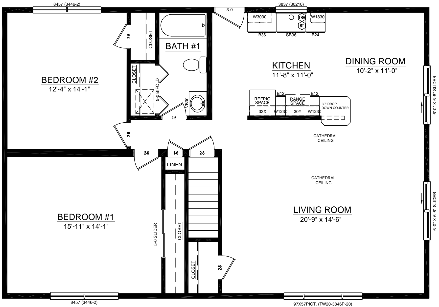
PLAN VIEW
