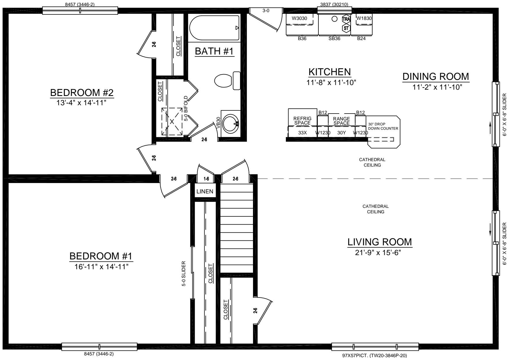
PLAN VIEW
