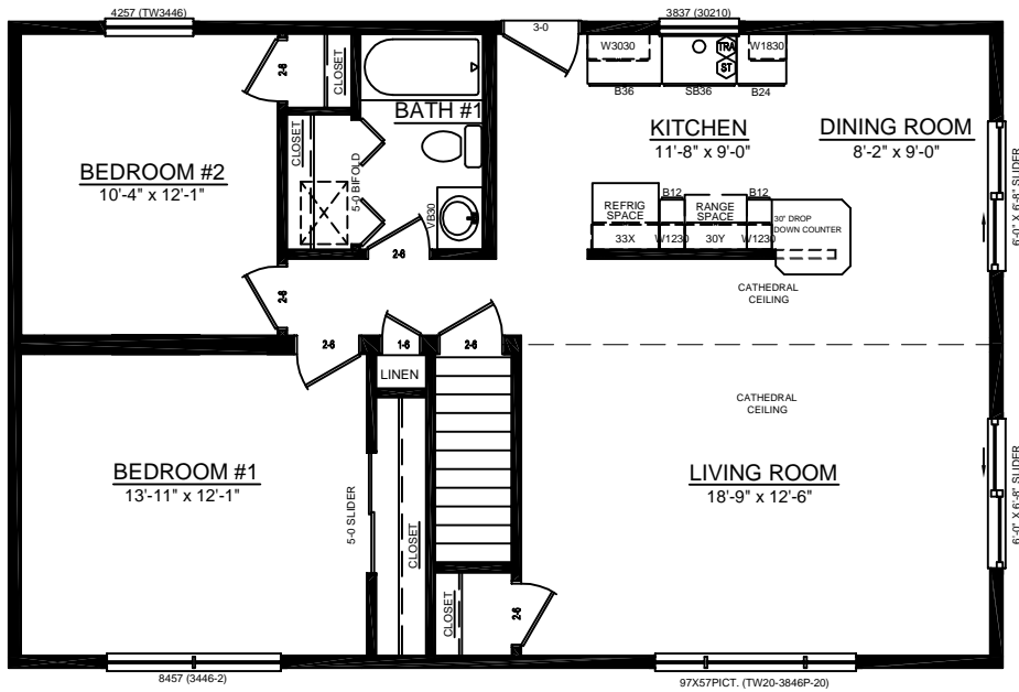
PLAN VIEW - 2 BEDROOM
