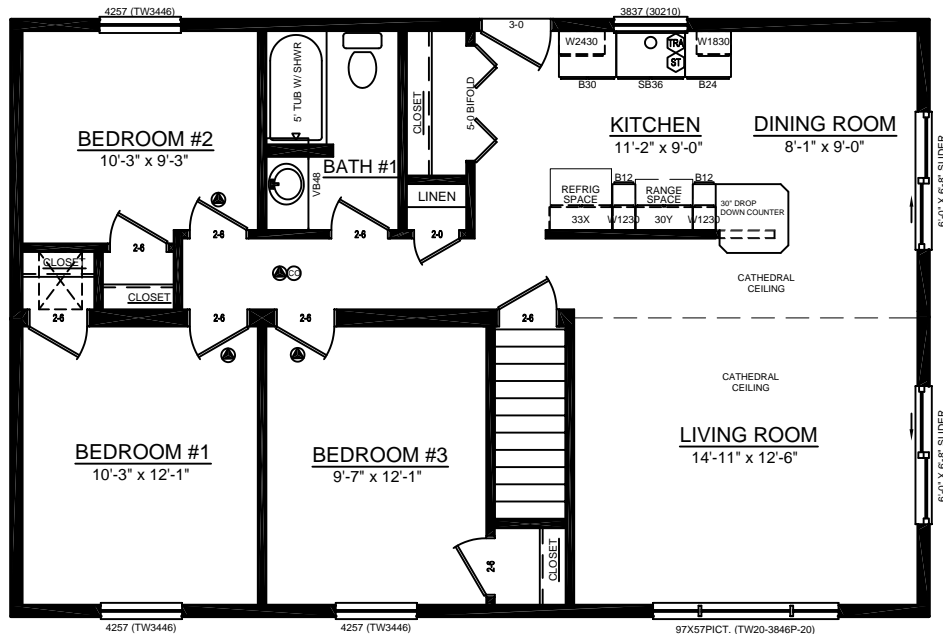
PLAN VIEW - 3 BEDROOM
