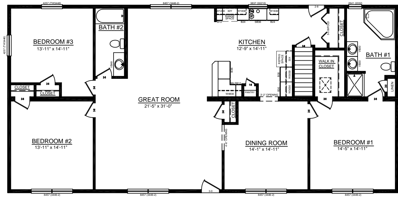
PLAN VIEW
