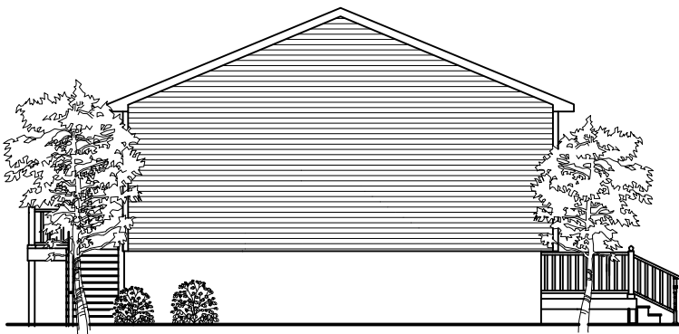
LEFT ELEVATION
