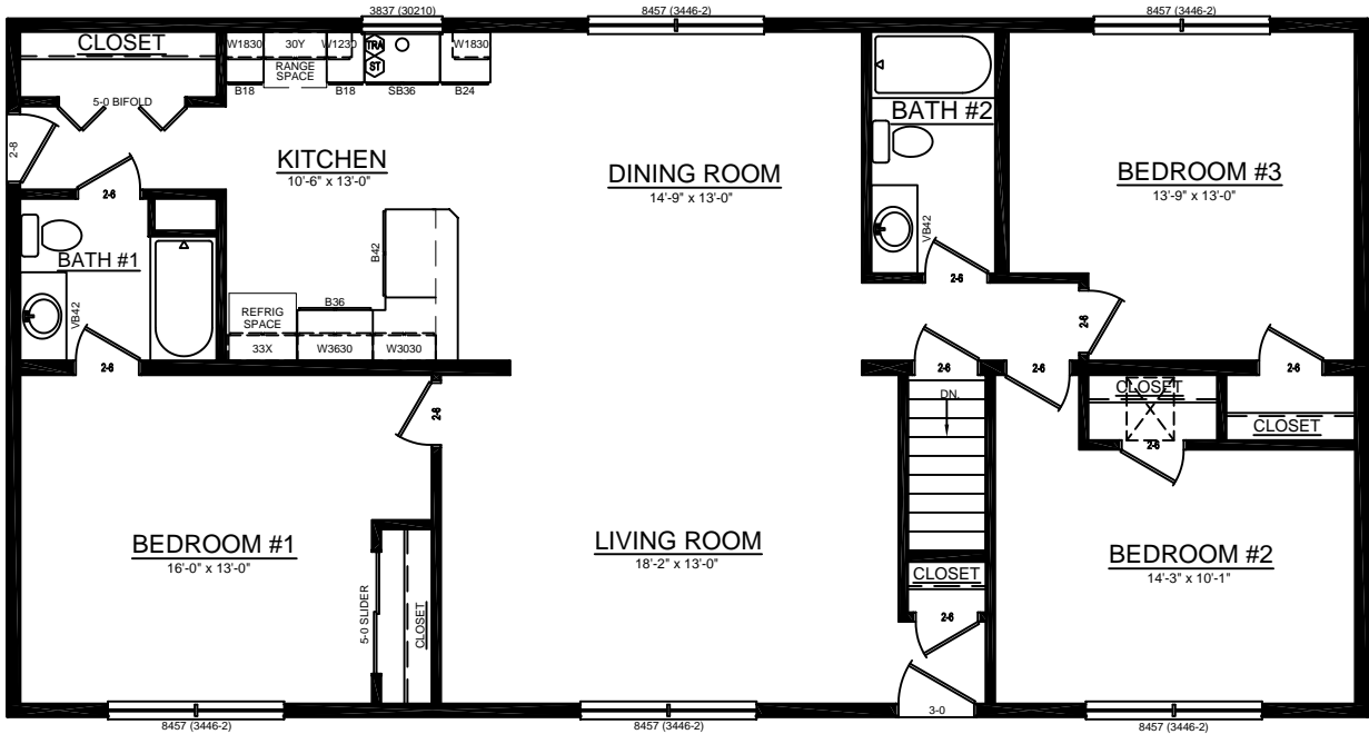
PLAN VIEW
