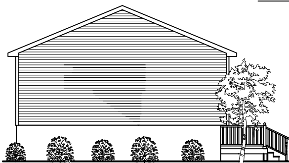
LEFT ELEVATION
