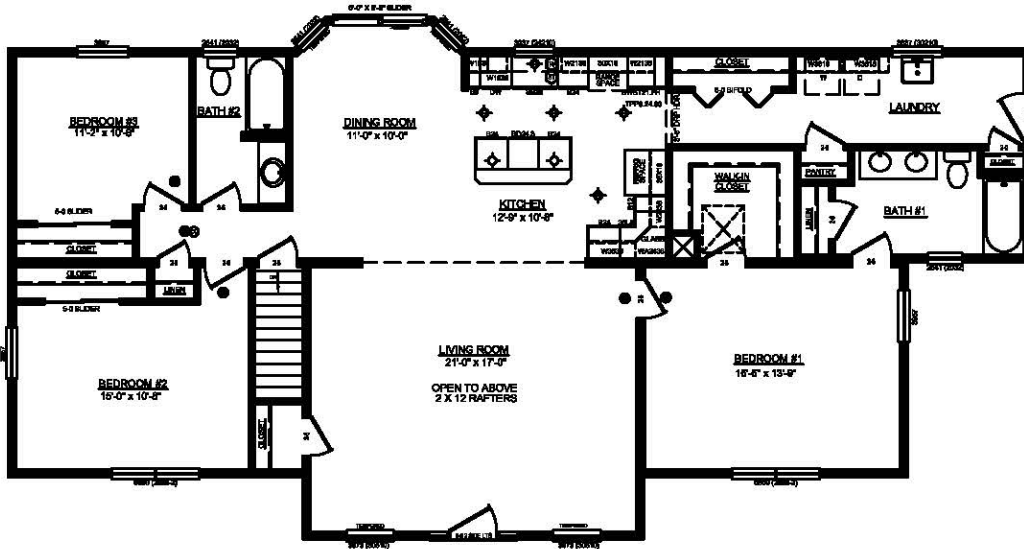
FLOOR PLAN
