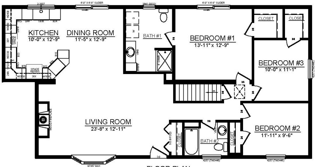
FLOOR PLAN
