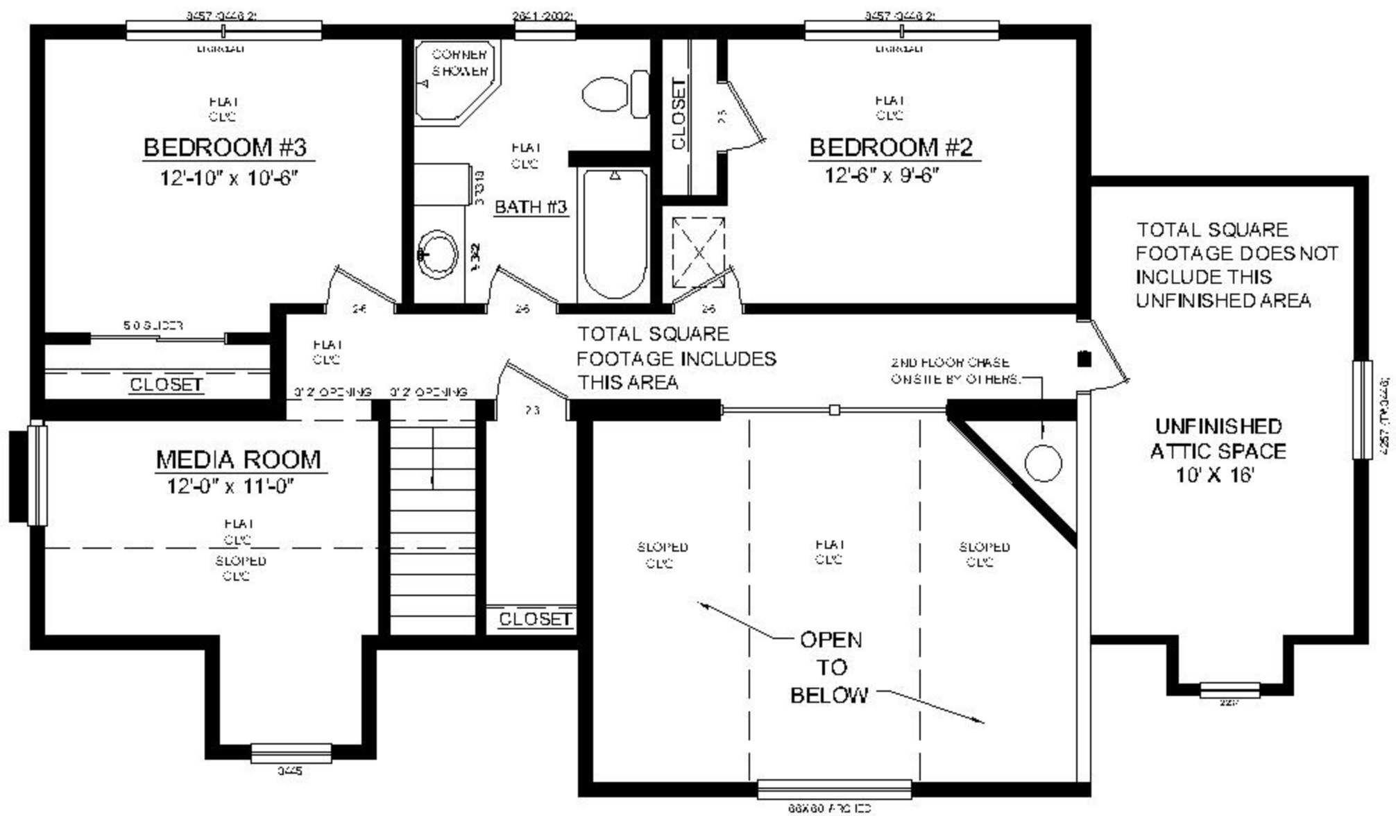
OPTIONAL SECOND FLOOR
