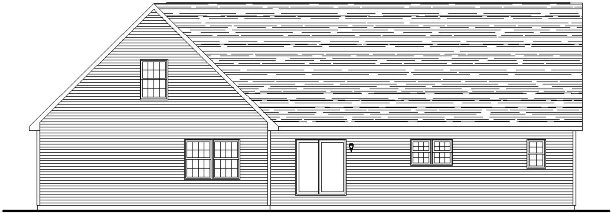
REAR ELEVATION
