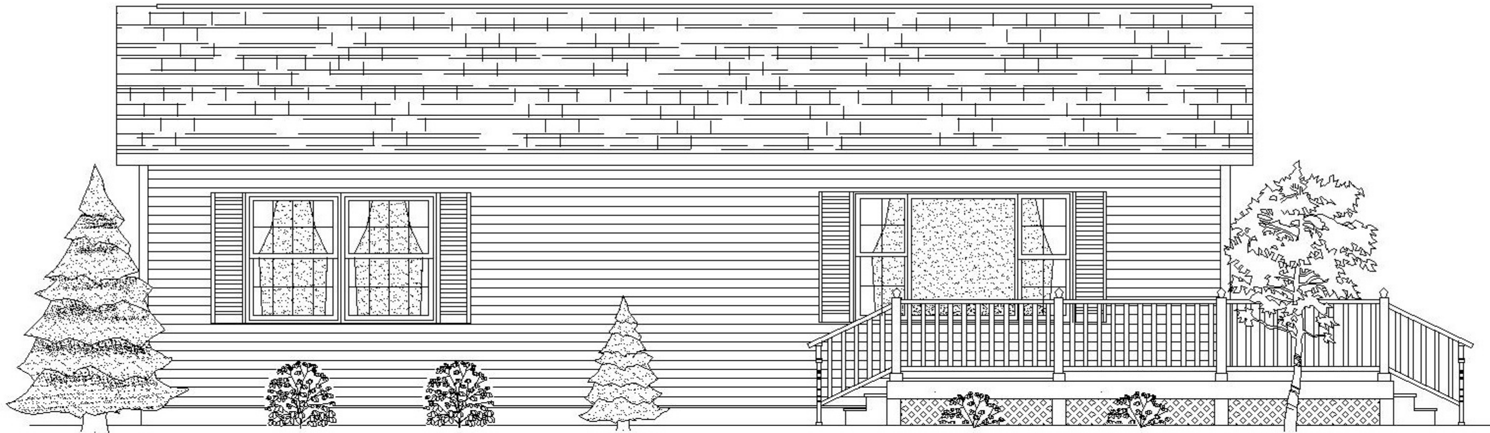
FRONT ELEVATION
